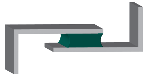
FIGURE 8.4 - LAP JOINT
