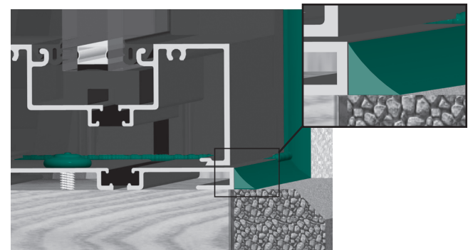
FIGURE 8.3 - FILLET JOINT
