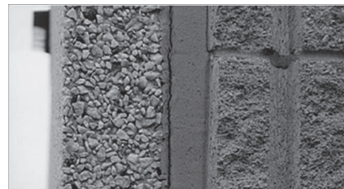
FIGURE 3.6a – SEALANT ADHESIVE BOND LOSS
