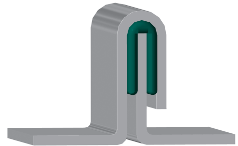
FIGURE 3.4 – LAP JOINT
